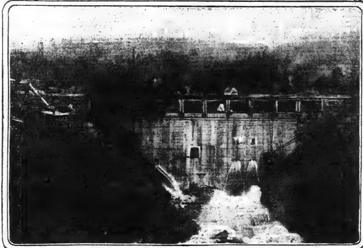
The completed Tallulah dam, photographed from the side of the gorge at a point below the lake, showing the water pouring through the sluice gates. On top of the dam is the public road, the site of the former bridge leading over the chasm being submerged by the lake. When the plant is in operation the water that remains from the tunnel flow, if there is any, will roll over the dam through the openings below the roadway.
